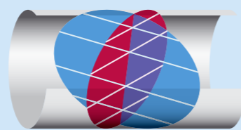
Multi-path measuring arrangement with crossed paths
